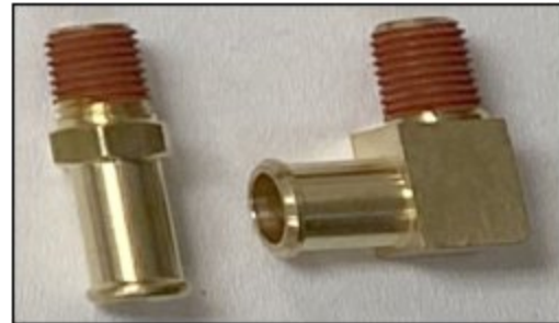
(1) FITT 1/4" NPT by 1/2" hose straight (1) FITT 1/4" NPT by 1/2" hose 90 degree
